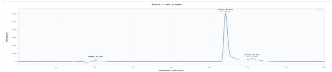
NAD+ 500mg - ND1-01: UV Chromatogram
