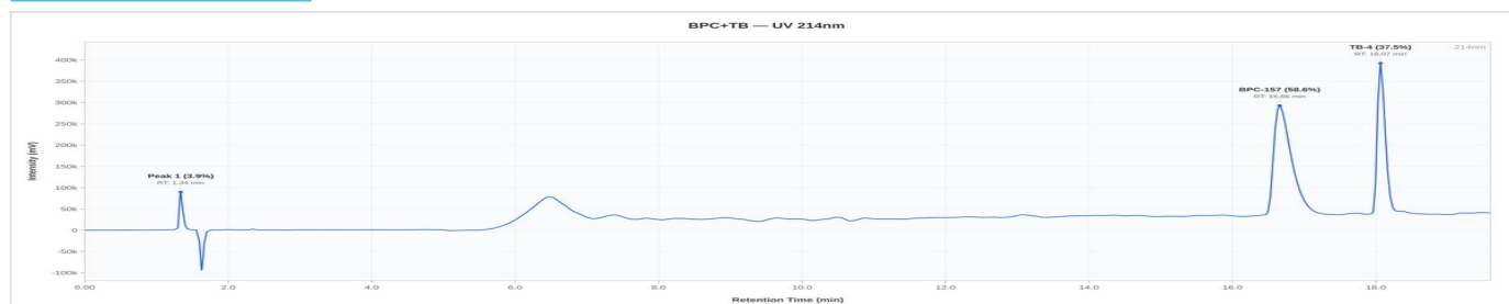
BPC+TB 10+10mg - BPTB20-04: UV Chromatogram
