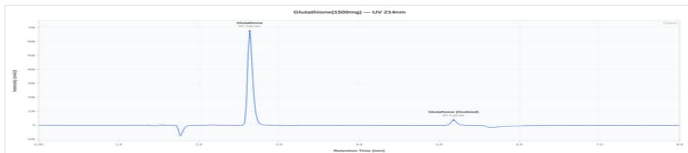
Glutathione 1500mg - GLUT-07: UV Chromatogram
